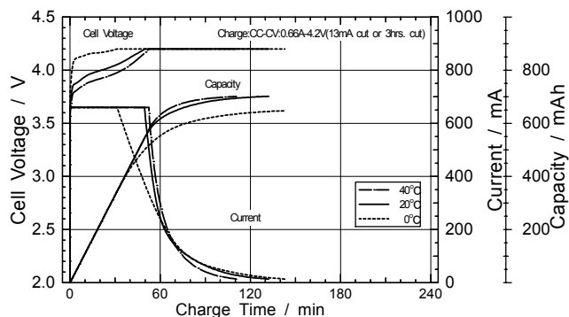
Charge characteristics
